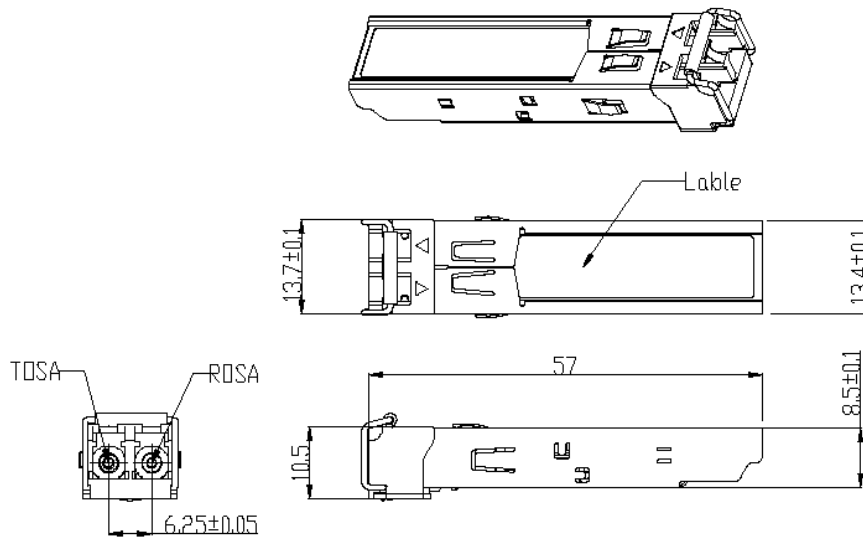
Figure 5. Mechanical Specifications
