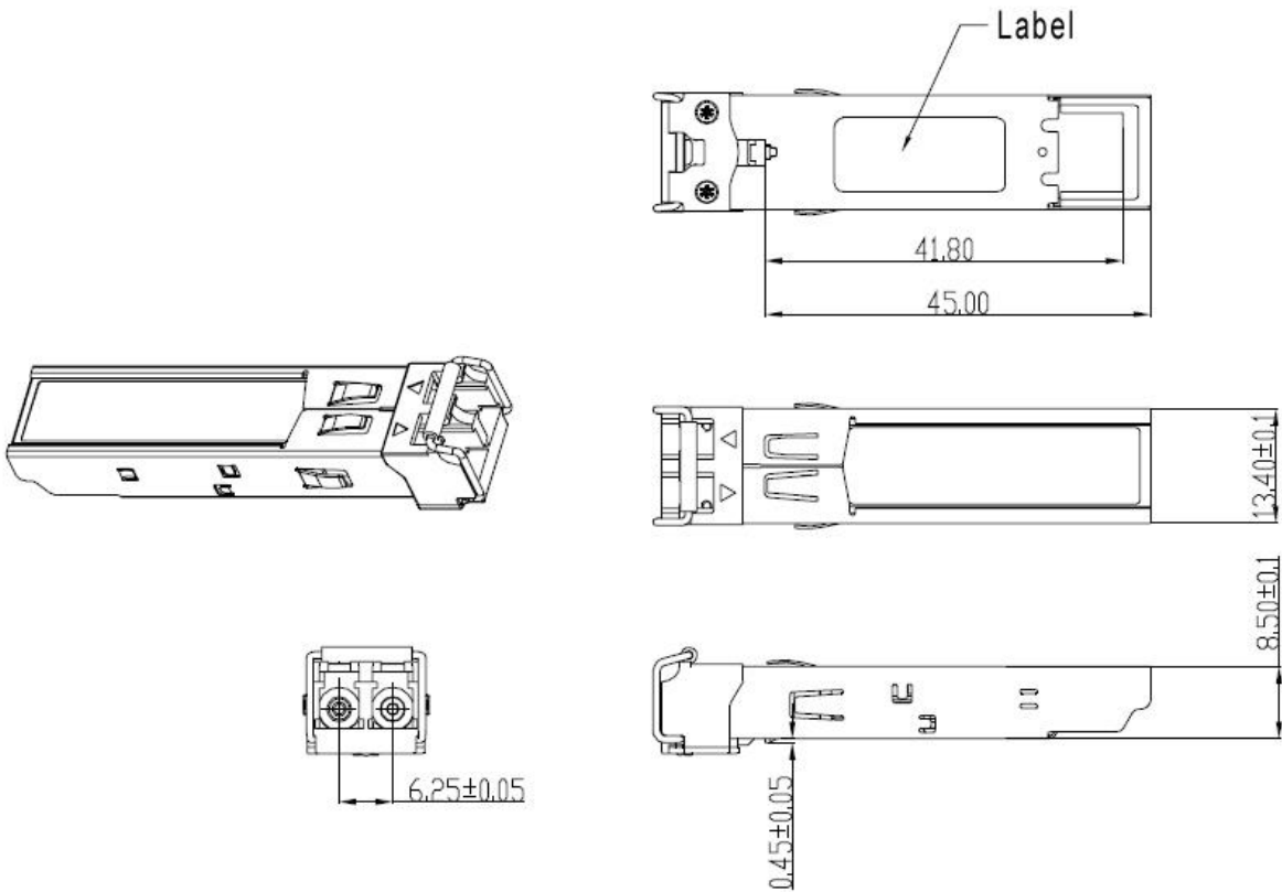
Figure 4. Mechanical Specifications
